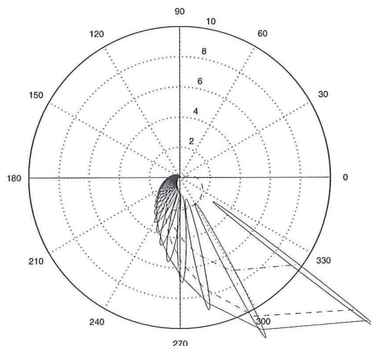
Figure 1: Frequency domain representation of \mathcal{D} in the Nyquist plane with ellipses U(\omega) at some frequencies, frequency response of \bar{G}(z) (dashdot), frequency response of G(z, \theta_{out}) (dashed) and frequency response of G(z, \theta_{bis}) (solid)
