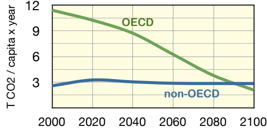
Fig.13: CO_2 emissions per capita for the period 2000-2100
