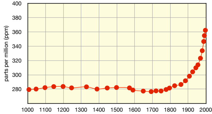
Fig.8: Atmospheric CO_2 concentrations (Law Dome ice core data before 1960, measurements at Mauna Loa observatory after 1960).
