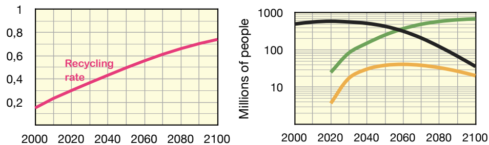
Fig.22: Left: Recycling rate of a-biotic material. Right: Employment (black: conventional sector, green: ecological sector, yellow: green technology sector)
