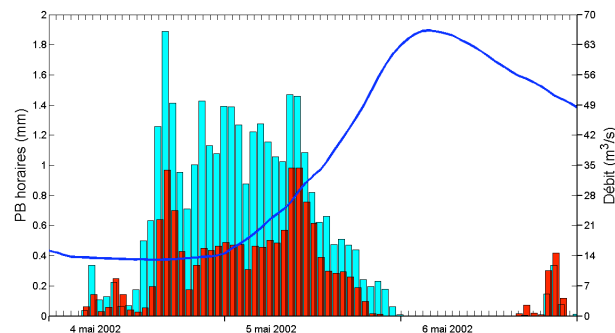
Fig. 9. Mean areal rainfall (mm) estimated from radar data (red) and from 14 rain gauges (blue-turquoise) for the Ourthe catchment at Tabreux (4-6 May 2002). The blue solid line represents the measured river flow (m 3 /s).
